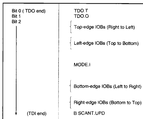
Figure 20: Boundary Scan Bit Sequence 66075_01
